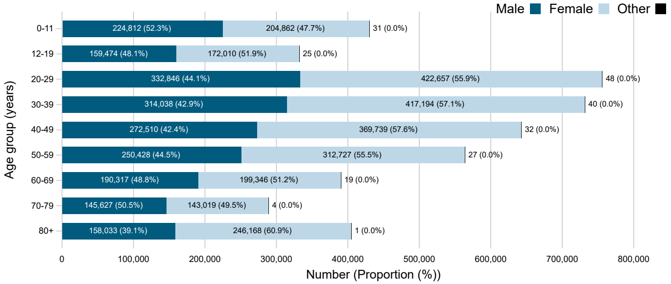
Figure 4a. Age and gender distribution of COVID-19 cases in Canada as of May 11, 2024 (n=4,536,034)
