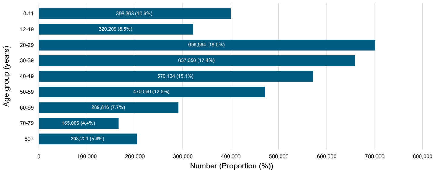
Figure 4. distribution of COVID-19 cases (n=3,774,052 1 ) in Canada as of July 4, 2022, 8 am EST 3
