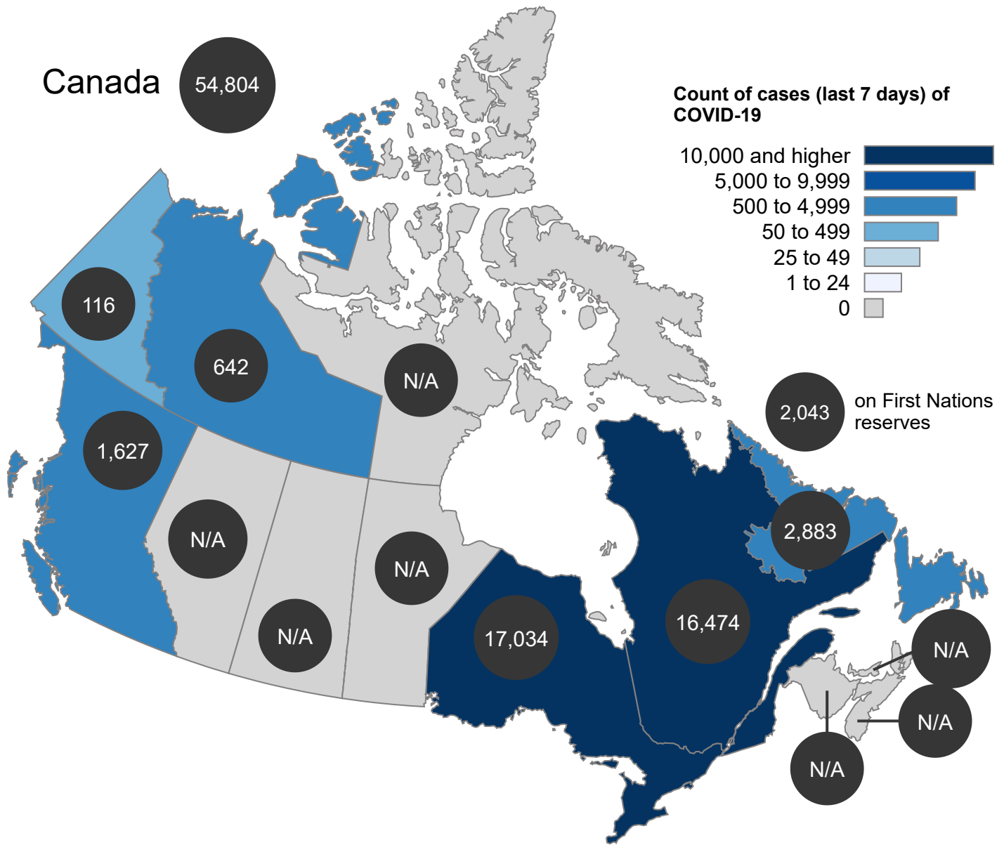
Figure 1a. Count of cases (last 7 days) of COVID-19, by province/territory as of March 31, 2022 (Last data update April 1, 2022, 9 am EST)
