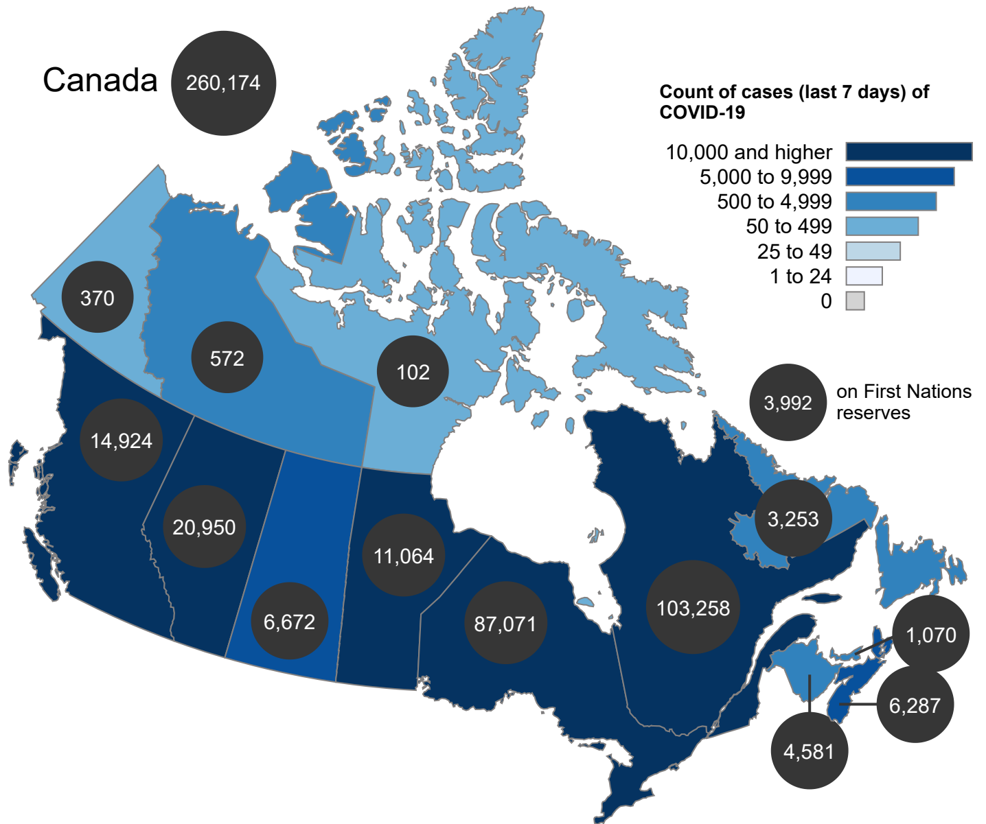
Figure 1a. Count of cases (last 7 days) of COVID-19, by province/territory as of January 9, 2022 (Last data update January 10, 2022, 8 am EST)
