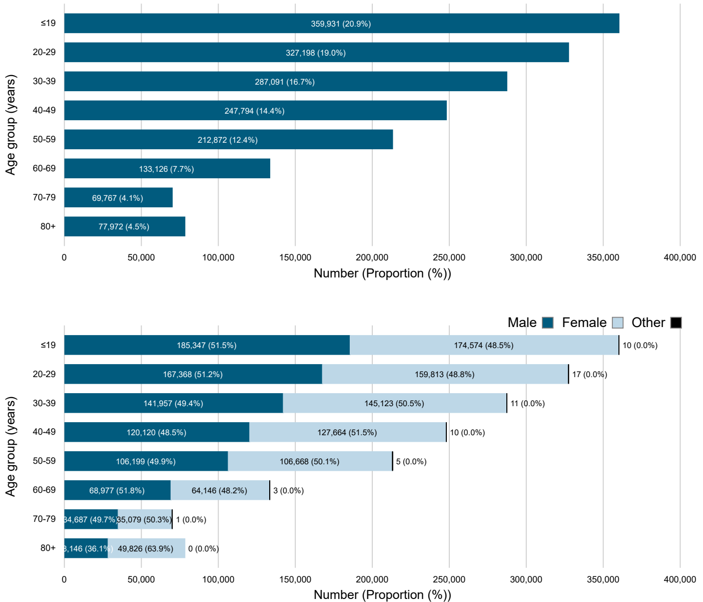
Figure 4. distribution of COVID-19 cases (n=1,718,937 1 ) in Canada as of November 5, 2021, 7 pm EST 4
