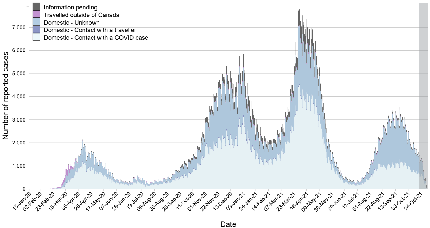
Figure 3. COVID-19 cases (n=1,276,770 1 ) in Canada by date 2 as of November 5, 2021, 7 pm EST (by exposure)
