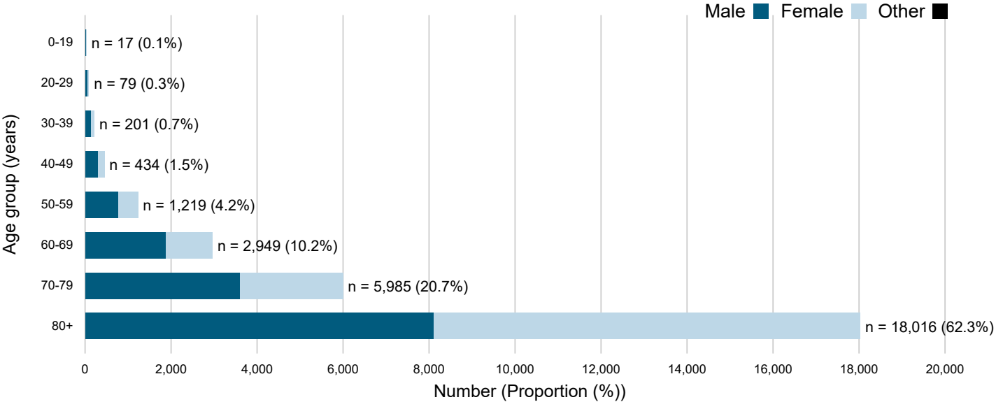
Figure 7c. Age and gender 4 distribution of COVID-19 cases deceased in Canada as of November 5, 2021, 7 pm EST (n=28,900 1 )
