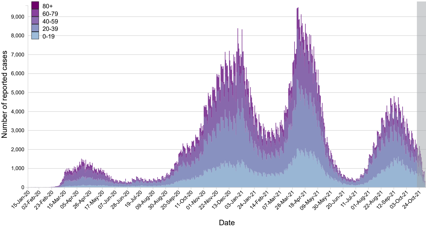
Figure 3. COVID-19 cases (n=1,640,307 1 ) in Canada by date 2 as of November 5, 2021, 7 pm EST (by age - 20 year groups)
