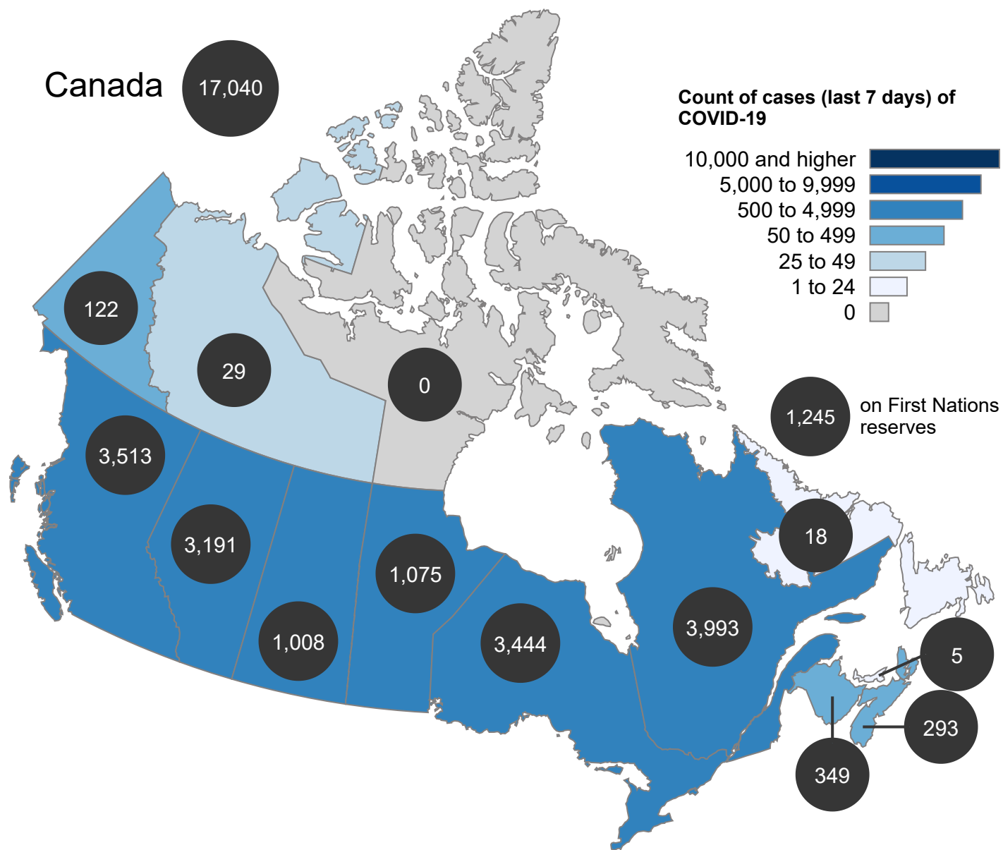
Figure 1a. Count of cases (last 7 days) of COVID-19, by province/territory as of November 9, 2021
