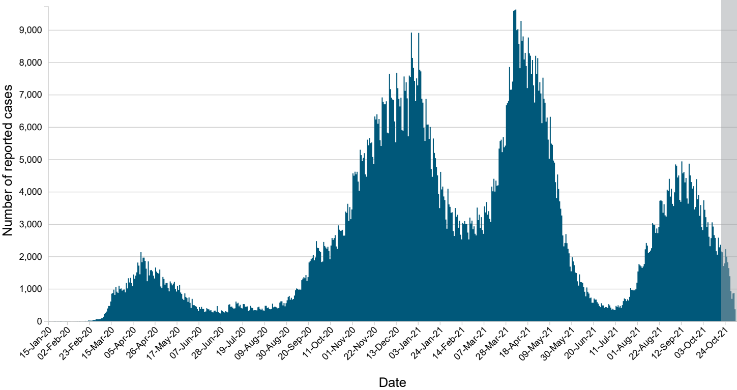
Figure 3. COVID-19 cases (n=1,718,937 1 ) in Canada by date 2 as of November 5, 2021, 7 pm EST (total cases)
