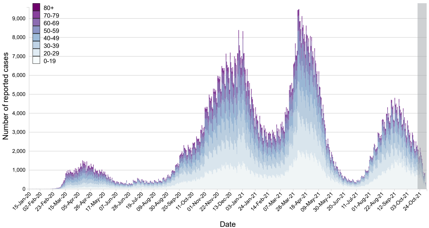
Figure 3. COVID-19 cases (n=1,640,307 1 ) in Canada by date 2 as of November 5, 2021, 7 pm EST (by age - 10 year groups)
