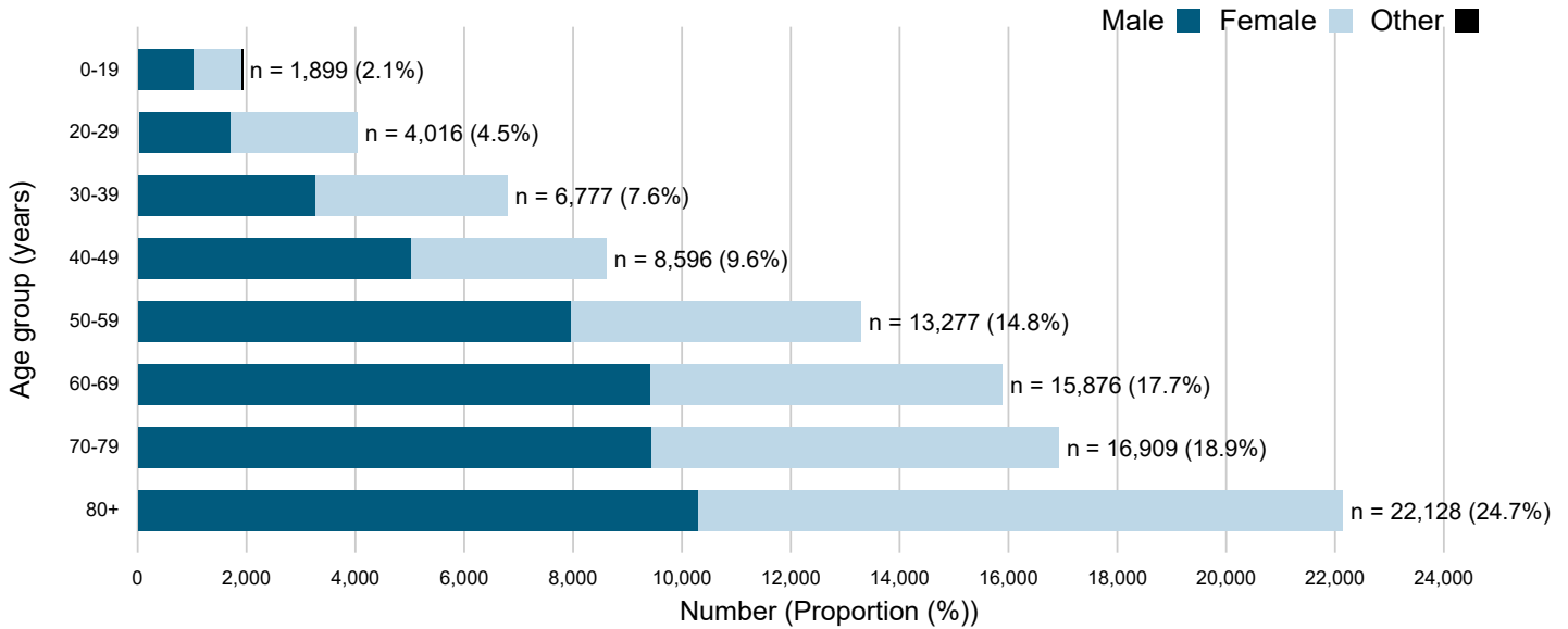
Figure 7a. Age and gender 4 distribution of COVID-19 cases hospitalized in Canada as of November 5, 2021, 7 pm EST (n=89,478 1 )
