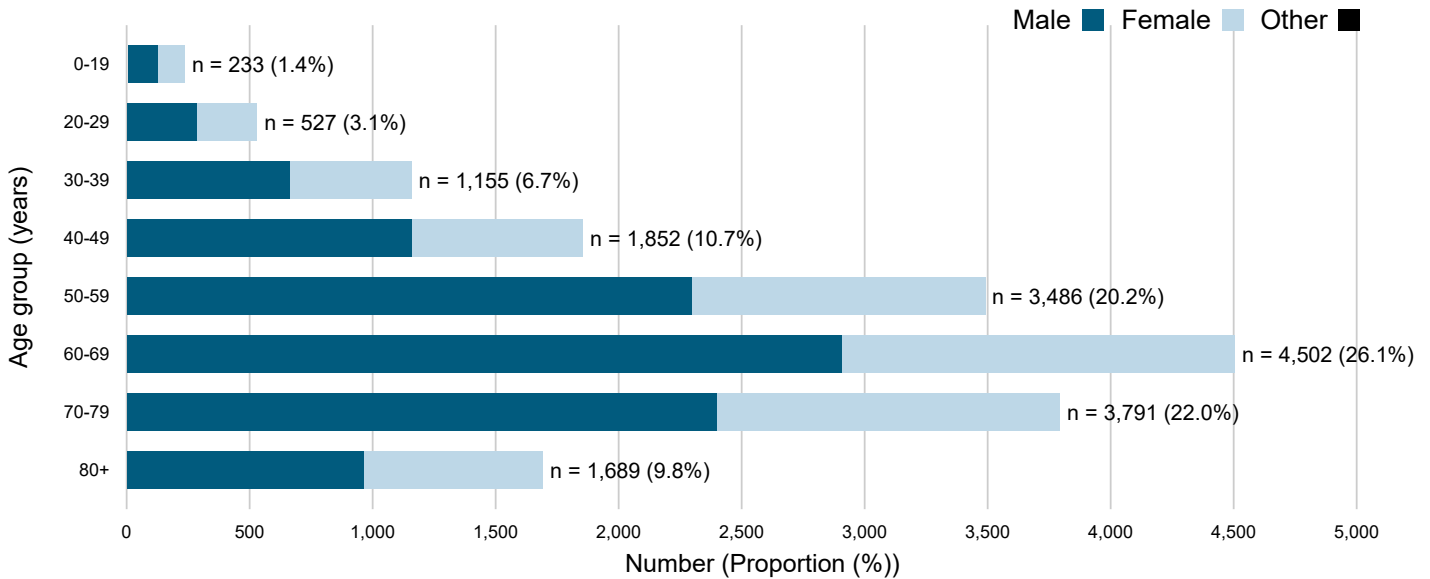
Figure 7b. Age and gender 4 distribution of COVID-19 cases admitted to ICU in Canada as of November 5, 2021, 7 pm EST (n=17,235 1 )
