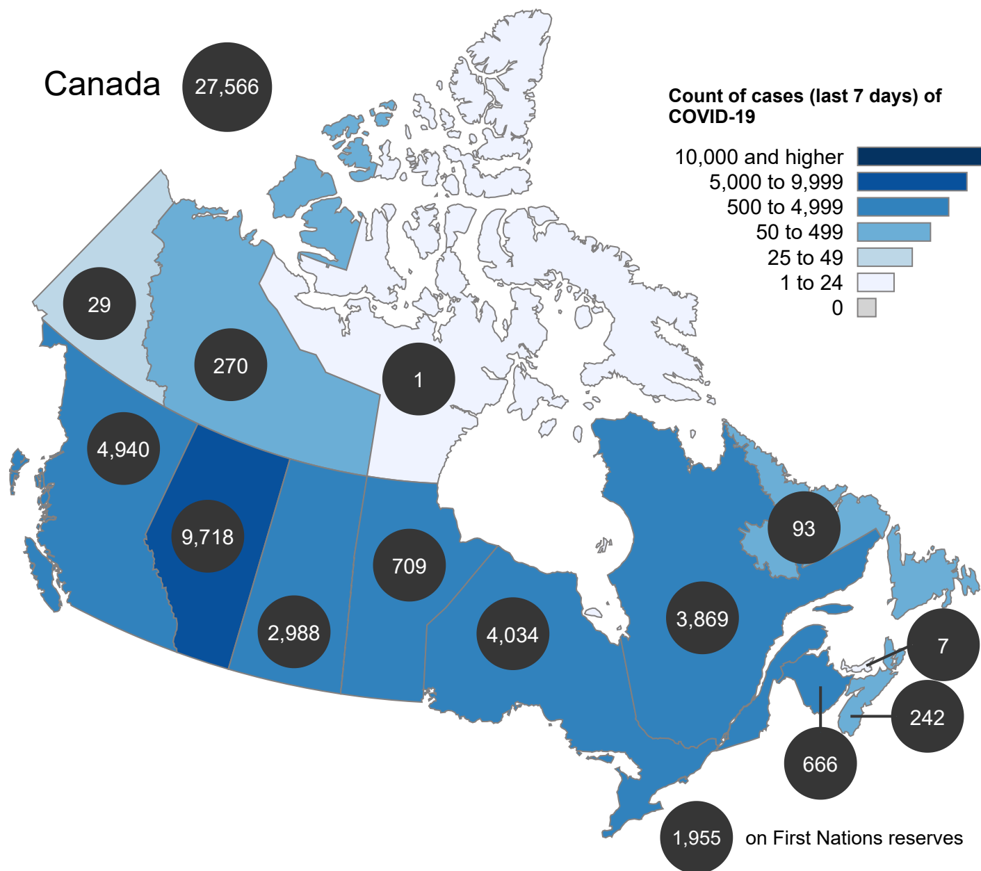
Figure 1a. Count of cases (last 7 days) of COVID-19, by province/territory as of October 5, 2021
