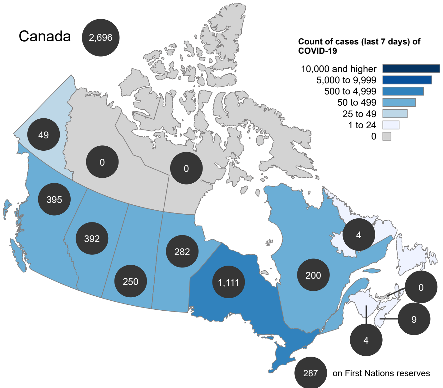
Figure 1a. Count of cases (last 7 days) of COVID-19, by province/territory as of July 25, 2021
